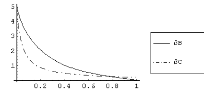
graphic 6 : \theta = 150
