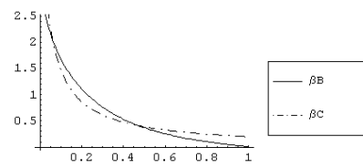
graphic 5 : \theta = 40
