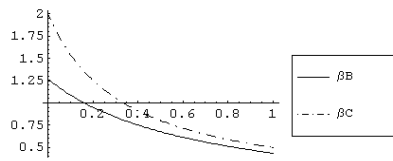
graphic 8 : \sigma_1^2 = \sigma_2^2 = 40
