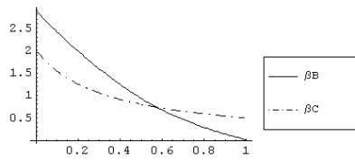
graphic 3: \theta = 100
