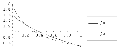
graphic 9 : \sigma_1^2 = \sigma_2^2 = 150
