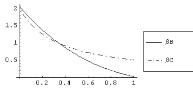
graphic 2: \theta = 40
