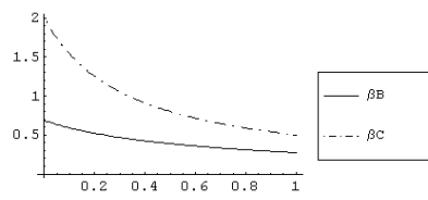
graphic 7 : \sigma_1^2 = \sigma_2^2 = 5
