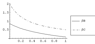
graphic 1: \theta = 5
