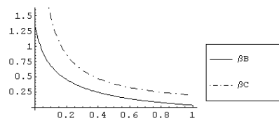
graphic 4 : \theta = 5
